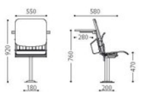
College FD chair with a fixed writing top measurements in mm
